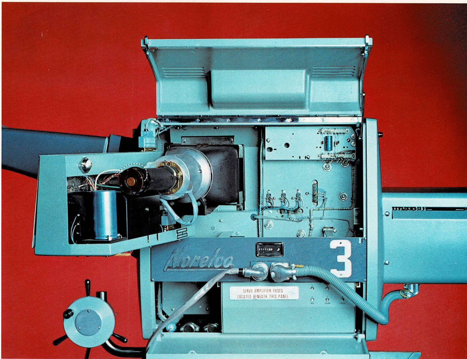
Camera head, right side open, showing swing-out viewfinder.
