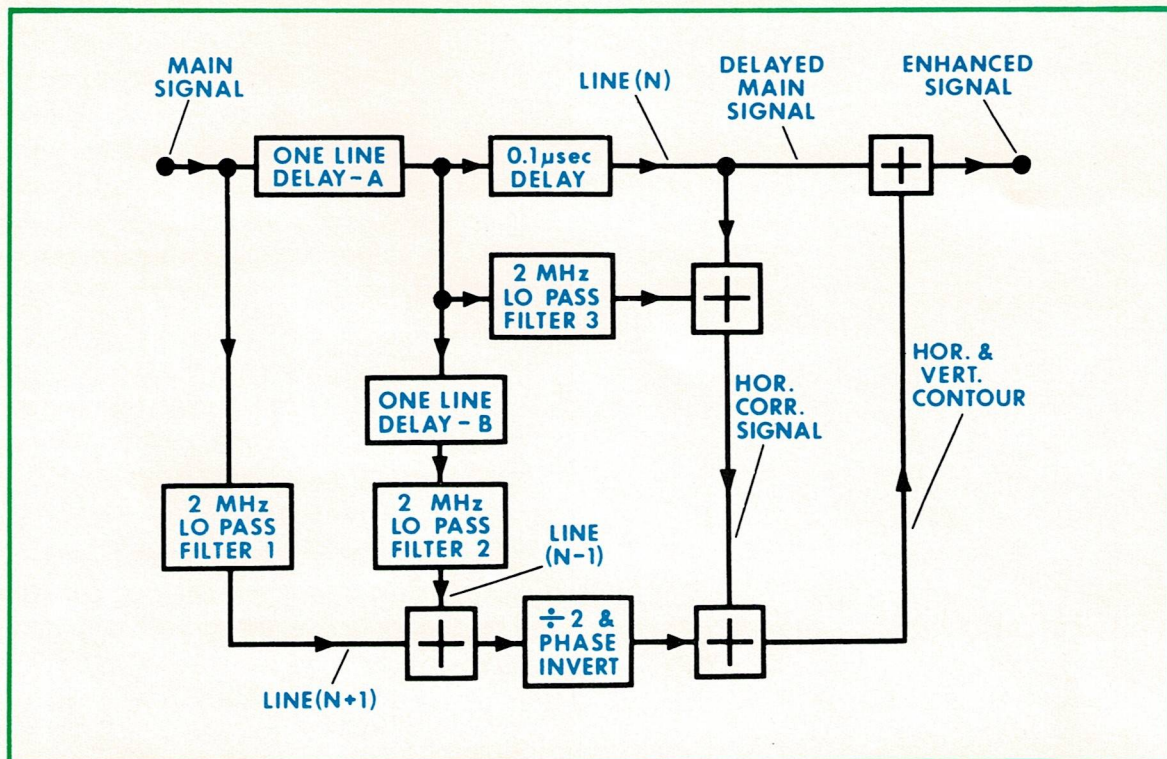
HORIZONTAL AND VERTICAL CONTOUR ENHANCER
