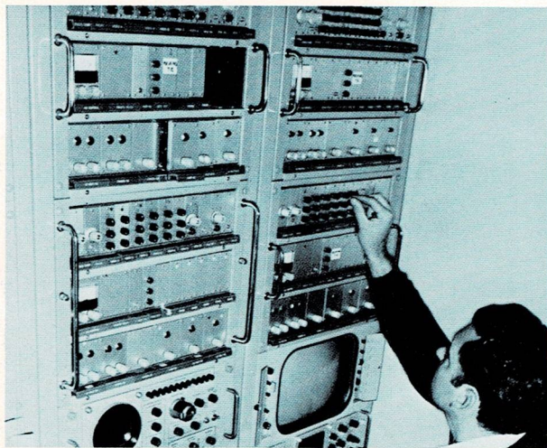
Compact installation—Four rack-mounted PC-70 Camera Control Units.
