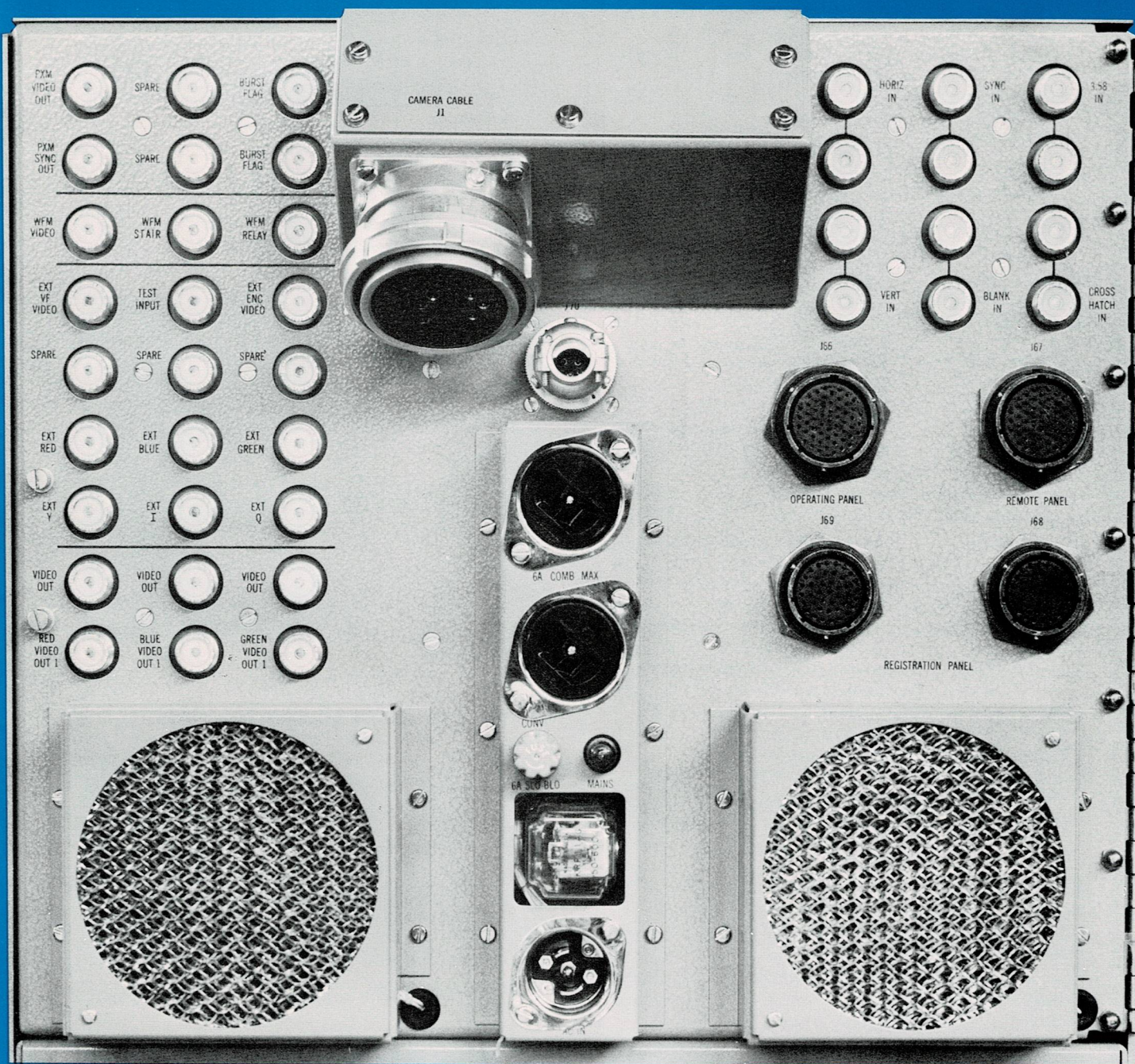
Rear view of PC-70 Electronics Unit.
