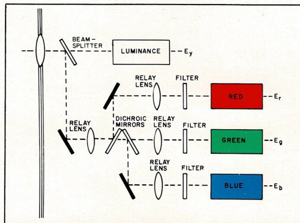
Typical optical system of four-tube color camera.
