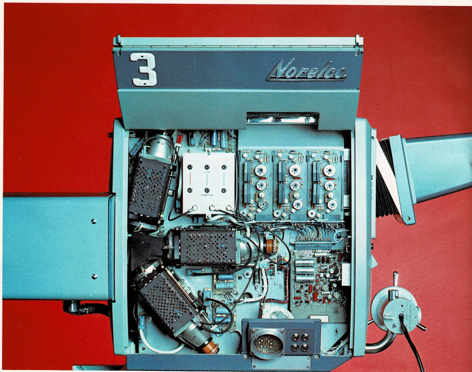
Camera head, left side open.
